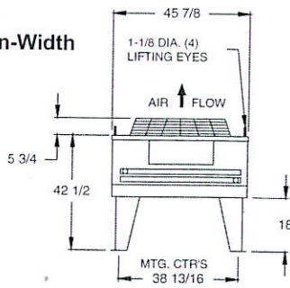
End View Double Fan-Width Units
