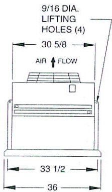
End View
